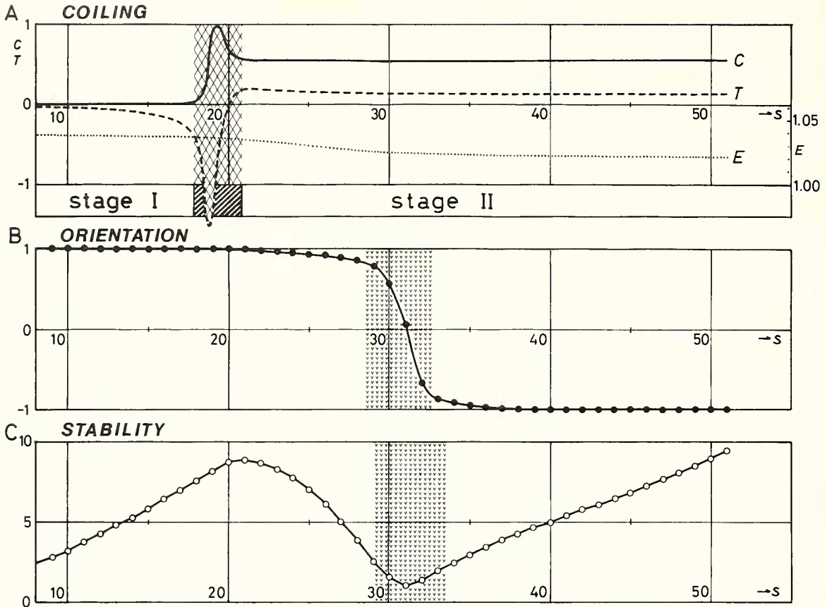
TEXT-FIG. 5. Diagrammatic figures showing change of some geometric and physical values during ontogeny of Eubostriyoceras muramotoi Matsumoto. A, moving frame analysis. B, Z component of unit vertical vector. C, length of vertical vector, a kind of stability index (see text).
